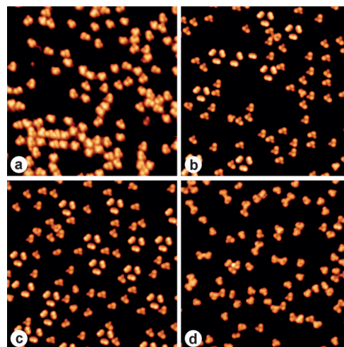
Figure 3. STM images ( T =5 K, 20×20 nm, 0.2 V, 2 nA) of 9-EP after a) deposition at 135 K and b) at 300 K. c), d) The same sample as in B after post-annealing for 10 min to 370 K and 490 K, respectively.
